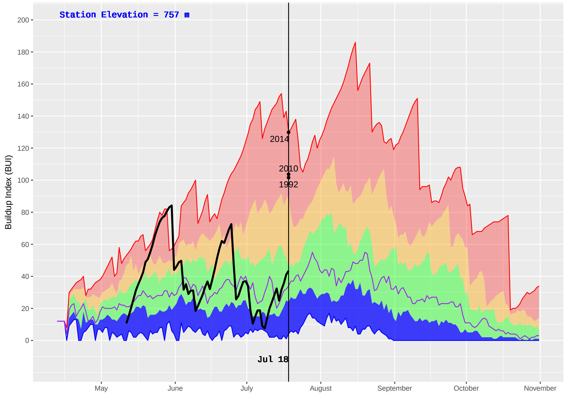
LEMORAY (140) : Historical (1988–2016) and Current (2018) Daily Buildup Index (BUI)
