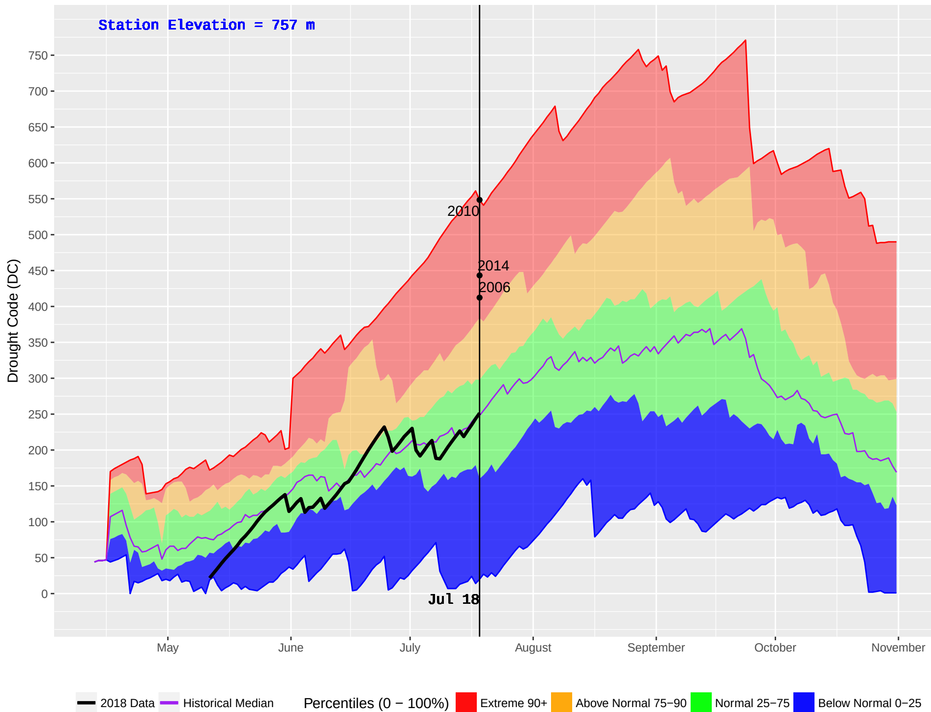
LEMORAY (140) : Historical (1988–2016) and Current (2018) Daily Drought Code (DC)
