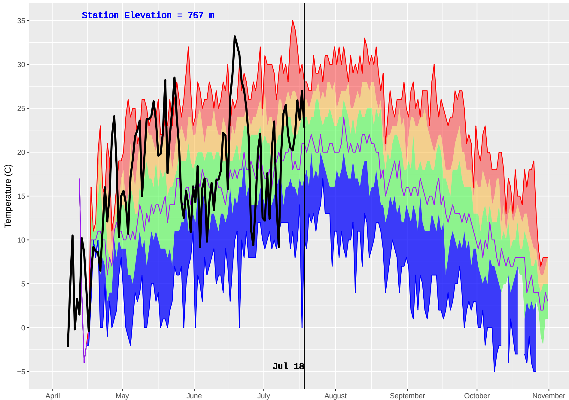
LEMORAY (140) : Historical (1988–2016) and Current (2018) Daily Temperature
