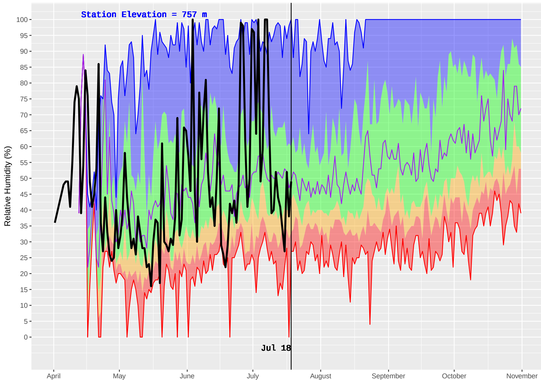
LEMORAY (140) : Historical (1988–2016) and Current (2018) Daily Relative Humidity
